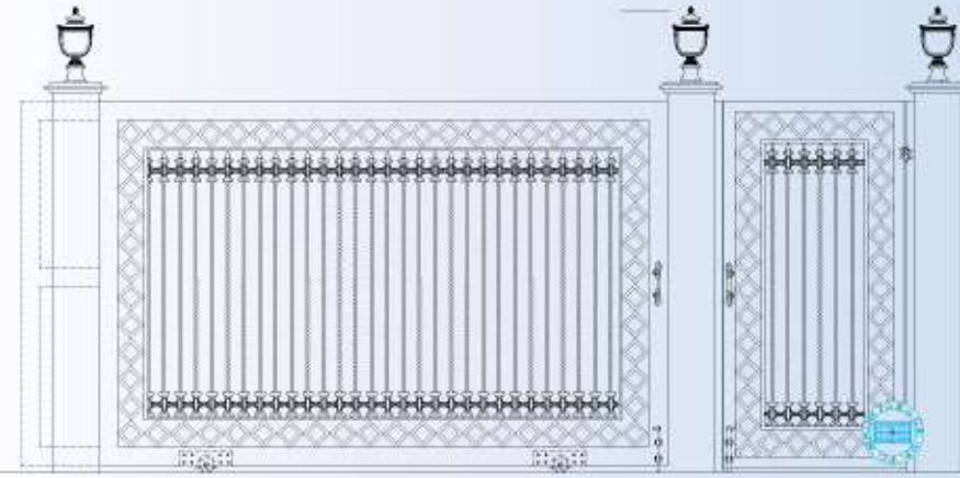
FRONT ELEVATION OF SLIDING WITH SWING GATE
