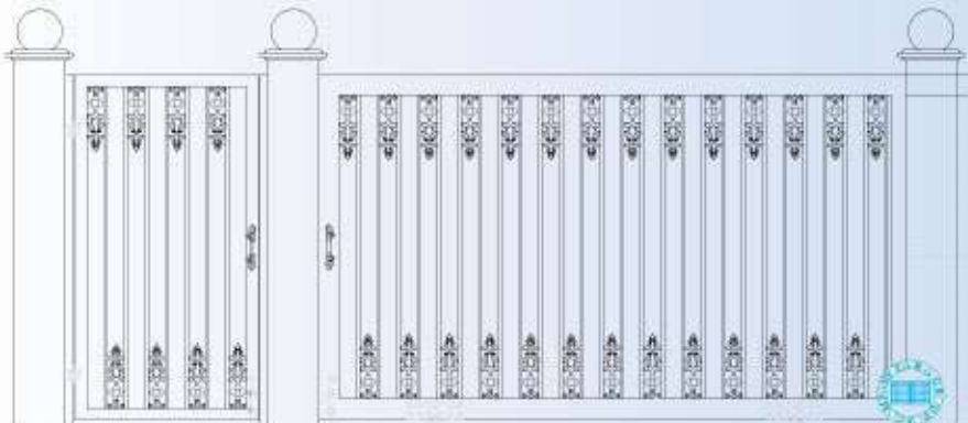
FRONT ELEVATION OF SLIDING WITH SWING GATE
