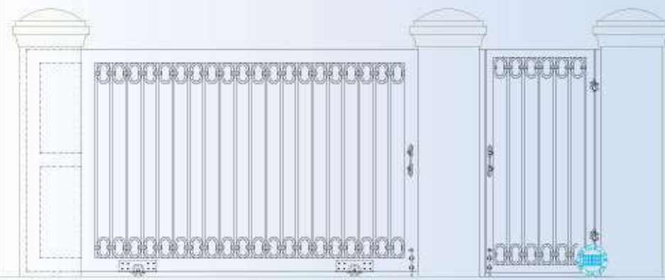
FRONT ELEVATION OF SLIDING WITH SWING GATE
