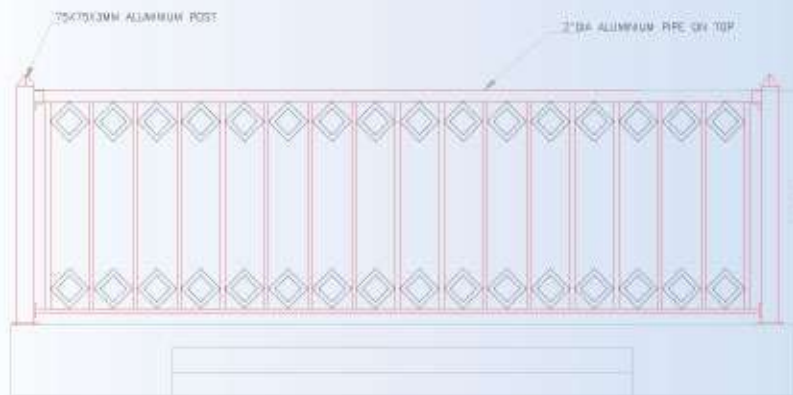
FRONT ELEVATION OF DECORATIVE BALCONY
