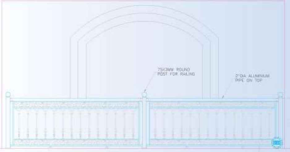
FRONT ELEVATION OF DECORATIVE BALCONY
