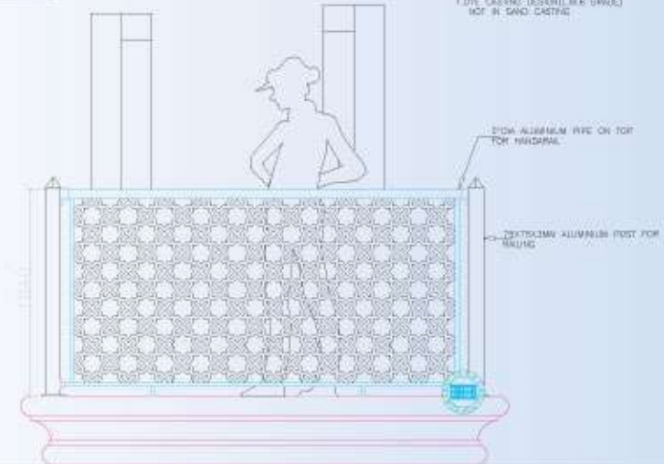
FRONT ELEVATION OF DECORATIVE BALCONY
